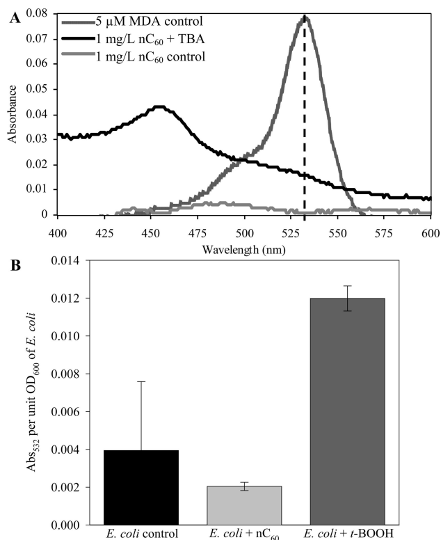
Figure 1. Assessment of lipid peroxidation in E. coli exposed to nC_{60} through the formation of colored adducts between MDA and TBA. (A) In the absence of cells, nC_{60} formed a colored product with TBA with increased absorption at 532 nm (dotted vertical line) as well as at other wavelengths. (B) After centrifuging the cells to remove most nC_{60} particles, E. coli incubated with nC_{60} showed no increase in absorption at 532 nm compared to the negative control, whereas the positive t -BOOH control exhibited increased absorbance due to lipid peroxidation.
